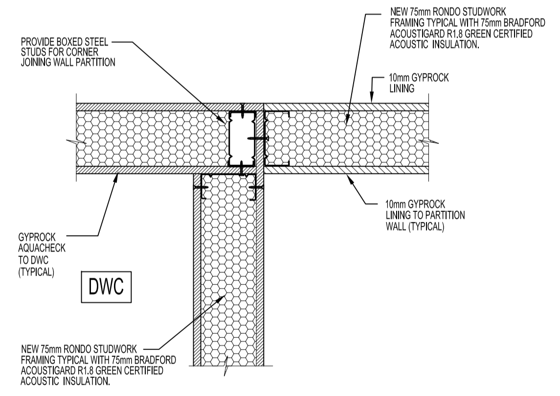
P1 PLAN DETAIL A1 SCALE 1:5
